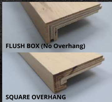
PRE-FABRICATED STAIR NOSINGS MATCHING ENGINEERED TIMBER FLOORING
